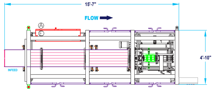
Standard Range Floorplan
